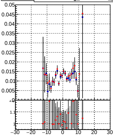
—●— tracking_iters01LST_DNN_1000events —●— tracking_iters01LST_preDNN_1000events
