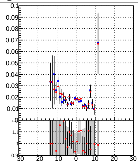
—●— tracking_iters01LST_DNN_1000events —●— tracking_iters01LST_preDNN_1000events
