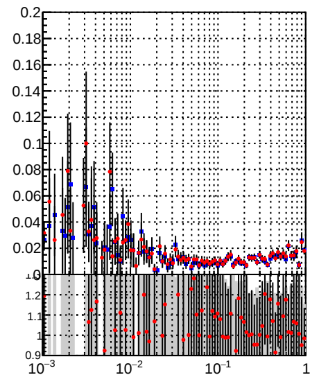
■ tracking_iters01LST_DNN_1000events ● tracking_iters01LST_preDNN_1000events
