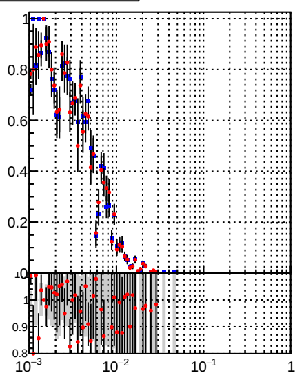
■ tracking_iters01LST_DNN_1000events ● tracking_iters01LST_preDNN_1000events
