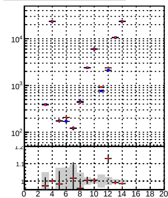
tracking_Iters01LST_DNN_1000events tracking_Iters01LST_preDNN_1000events
