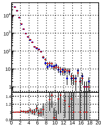
N of reco track vs. \chi^2 for tracking_iters01LST_DNN_1000events vs tracking_iters01LST_preDNN_1000events
