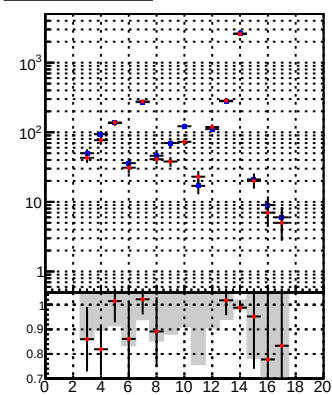
tracking_Iters01LST_DNN_1000events tracking_Iters01LST_preDNN_1000events
