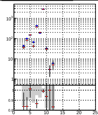
tracking_Iters01LST_DNN_1000events tracking_Iters01LST_preDNN_1000events
