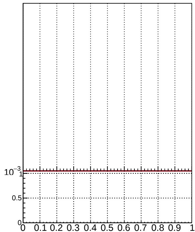
RecoPVAssoc2GenPVNotMatched_Missing
