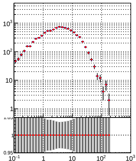
tracking_iters01LST_DNN_1000events N of simulated tracks vs pT tracking_iters01LST_preDNN_1000events
