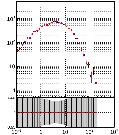
tracking_iters01LST_DNN_1000events tracking_iters01LST_preDNN_1000events
