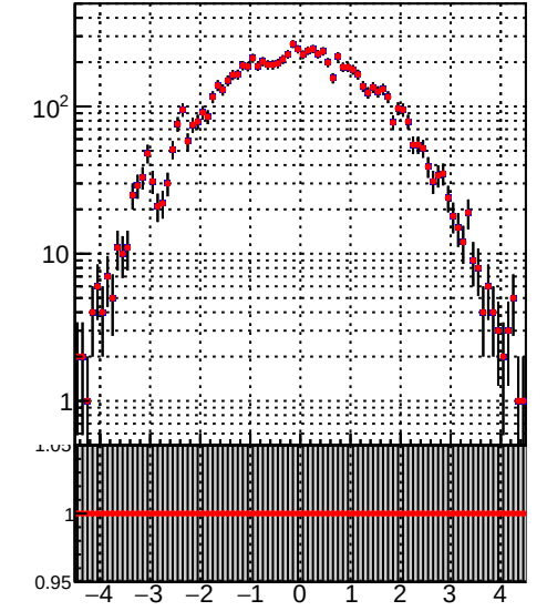
tracking_iters01LST_DNN_1000events tracking_iters01LST_preDNN_1000events
