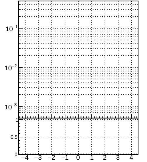
tracking_iters01LST_DNN_1000events tracking_iters01LST_preDNN_1000events
