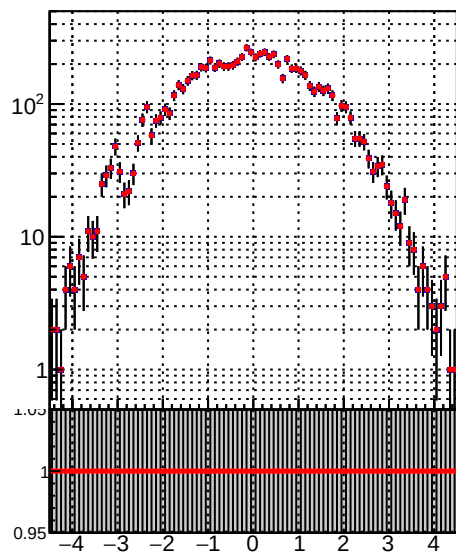
tracking_iters01LST_DNN_1000events tracking_iters01LST_preDNN_1000events
