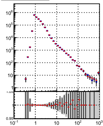
tracking_Iters01LST_DNN_1000events tracking_Iters01LST_preDNN_1000events
