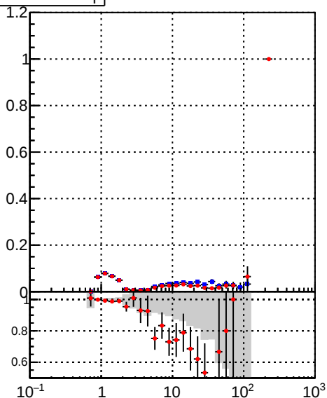
— tracking_iters01LST_DNN_1000events — tracking_iters01LST_preDNN_1000events
