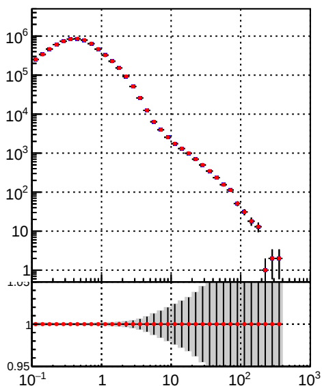
tracking_iters01LST_DNN_1000events tracking_iters01LST_preDNN_1000events
