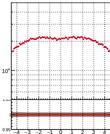
tracking_iters01LST_DNN_1000events tracking_iters01LST_preDNN_1000events
