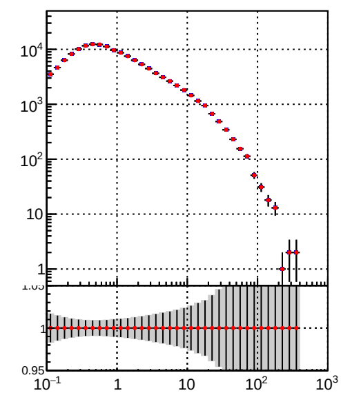
tracking_iters01LST_DNN_1000events tracking_iters01LST_preDNN_1000events
