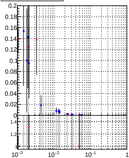
■ tracking_Iters01LST_DNN_1000events ● tracking_Iters01LST_preDNN_1000events
