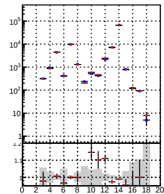
tracking_Iters01LST_DNN_1000events tracking_Iters01LST_preDNN_1000events
