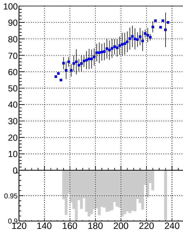
MatchedRecoVtx_vs_GenVtx
