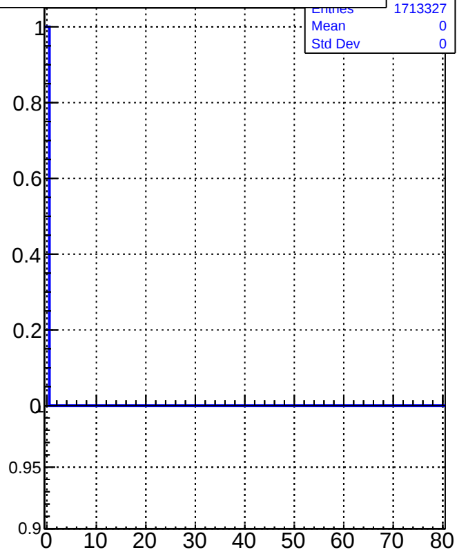
tracking_iters01LST
