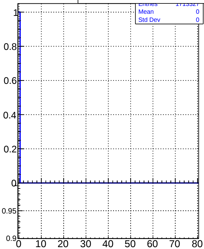
tracking_iters01LST
