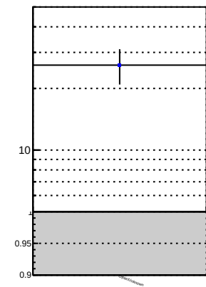
N of reco track vs. \chi^2 overSet
