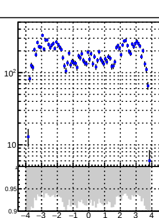
N of associated (recoToSim) duplicate tracks vs eta
