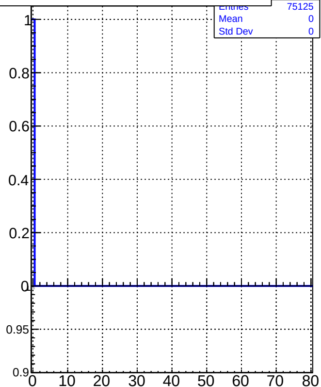
tracking_iters01LST
