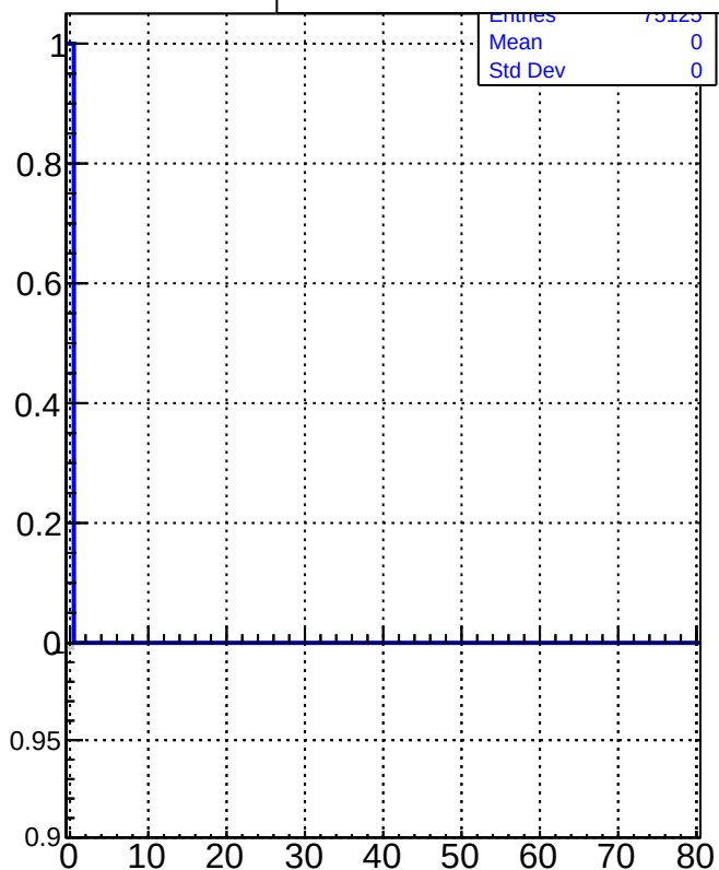
tracking_iters01LST
