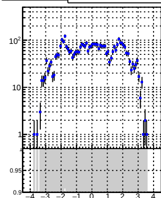
N of reco track vs \eta tracking_iters01LST
