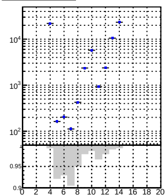
N of reco track vs hit tracking_Iters01LST
