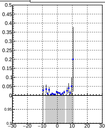
Fake rate vs \nu tracking_Iters01LST
