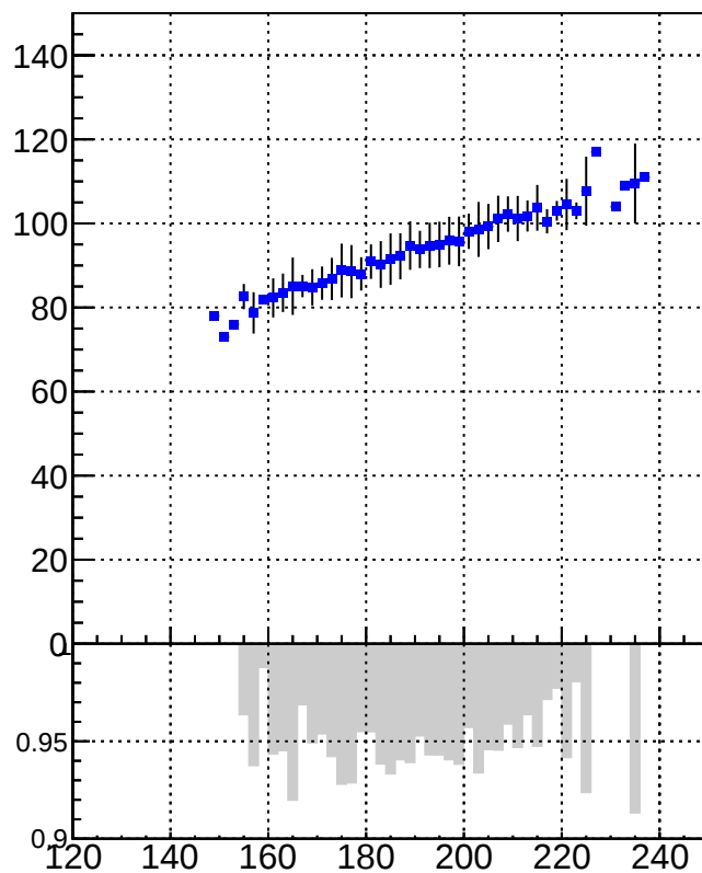
MatchedRecoVtx_vs_GenVtx
