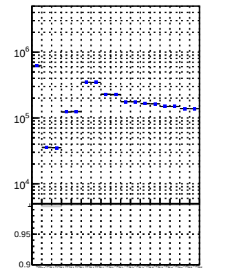
N of reco track vs. \chi^2 tracking_iters01LST
