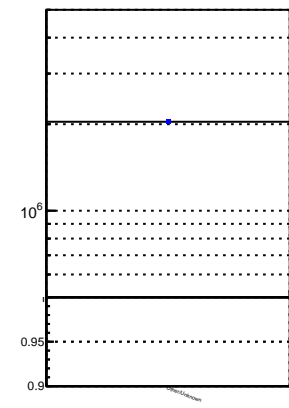
N of reco track vs. \chi^2 tracking_lters01LST
