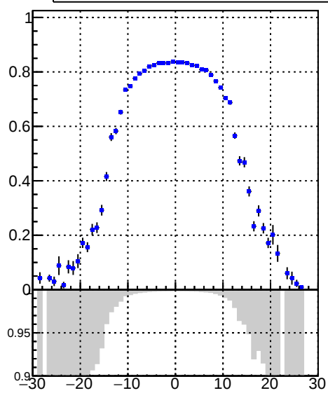
Efficiency vs. tracking_iters01LST
