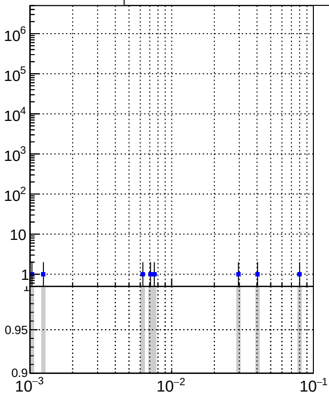
N of simulated tracks vs dR
