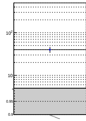
N of reco track vs. \chi^2 overSet
