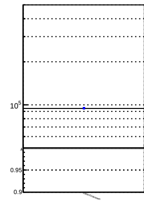
N of reco track vs. \chi^2 tracking_Iters01LST
