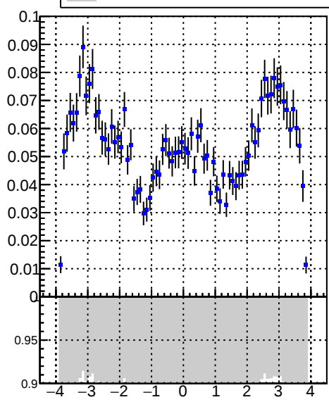
tracking_iters01LST_DNN_1000events
