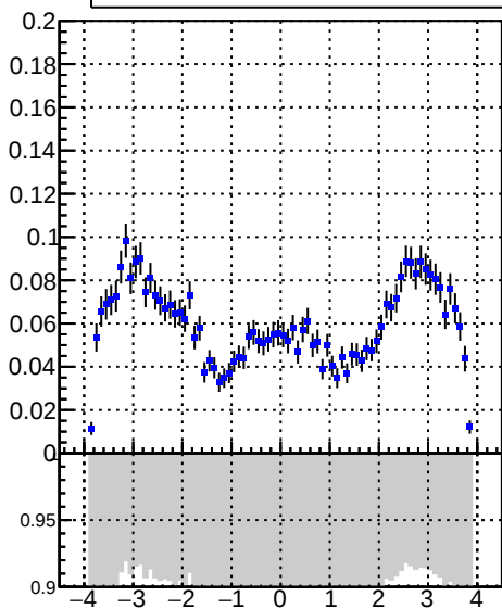
tracking_lters01LST_DNN_1000events
