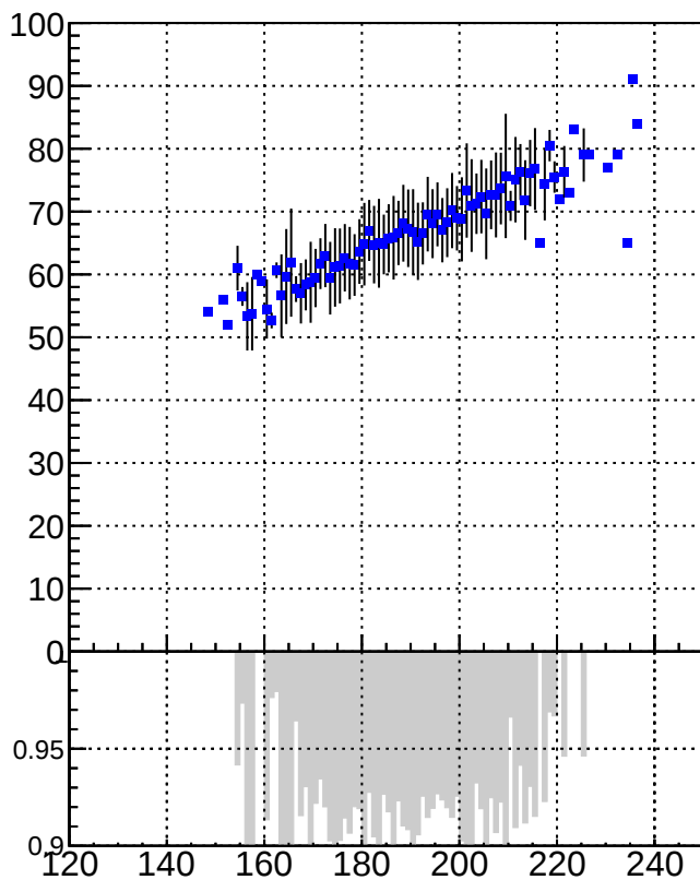
RecoVtx_vs_GenVtx
