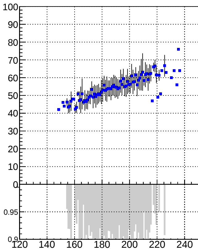
RecoVtx_vs_GenVtx
