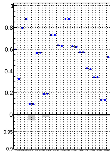
Fake rate vs. tracking_iters01LST_DNN_1000events
