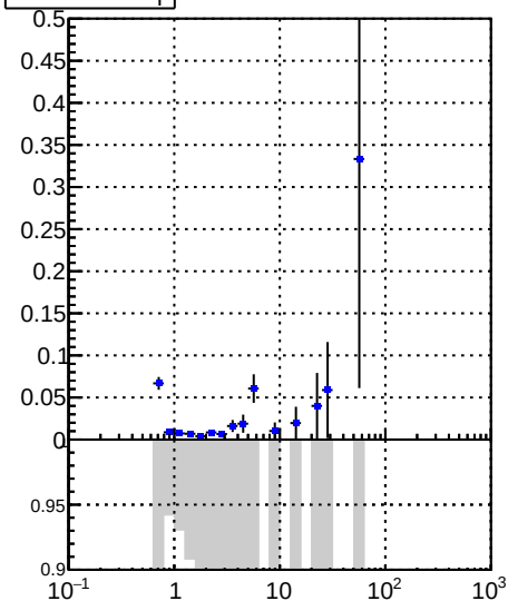
tracking_Iters01LST_DNN_1000events
