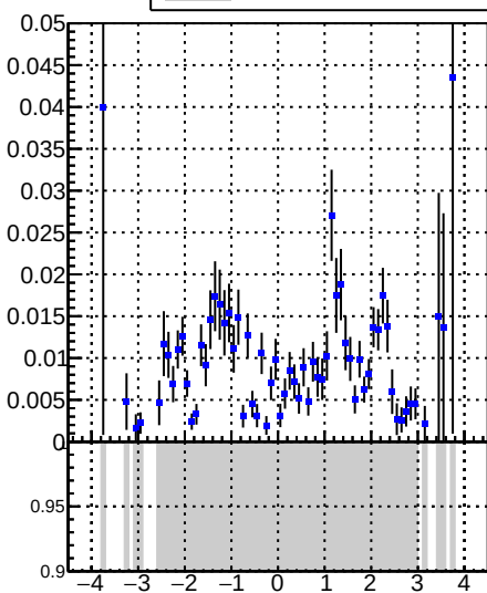
tracking_Iters01LST_DNN_1000events
