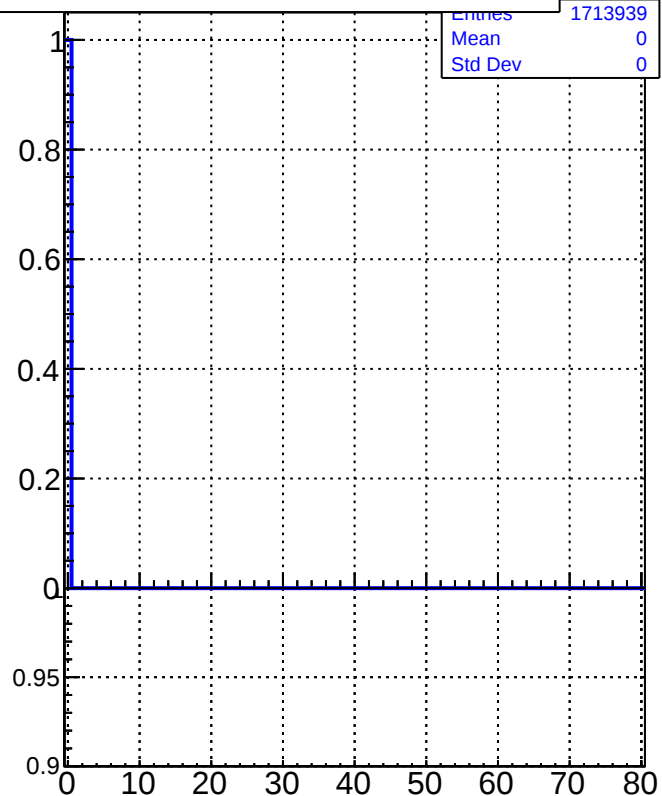
tracking_iters01LST_DNN_1000events
