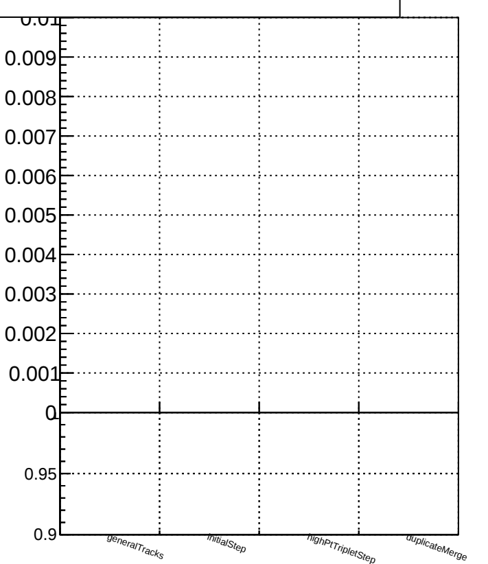
tracking_Iters01LST_DNN_1000events
