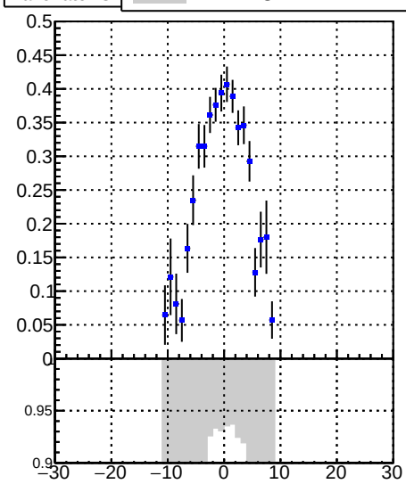
Fake rate vs vertpos tracking_iters01LST_DNN_1000events
