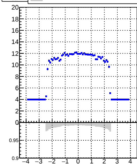
mean hit tracking_Iter01LST_DNN_1000events
