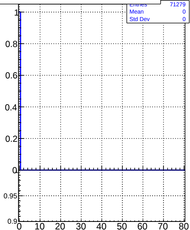
tracking_iters01LST_DNN_1000events
