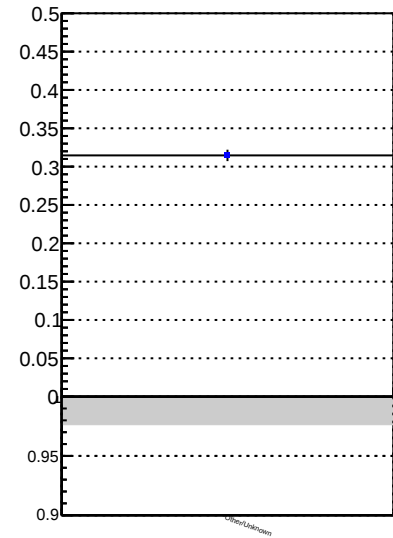
Fake rate vs. —●— tracking_iters01LST_DNN_1000events
