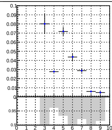
tracking_Iters01LST_DNN_1000events
