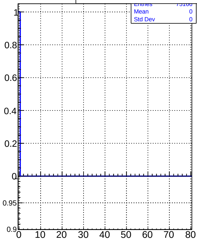
tracking_iters01LST_DNN_1000events
