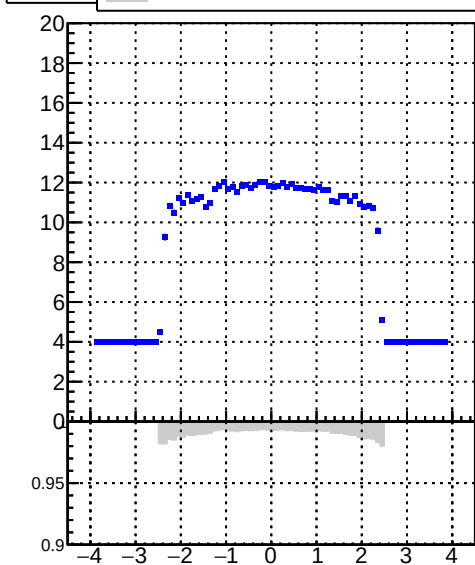
mean hit tracking_Iters01LST_DNN_1000events
