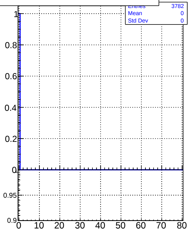
tracking_iters01LST_DNN_1000events
