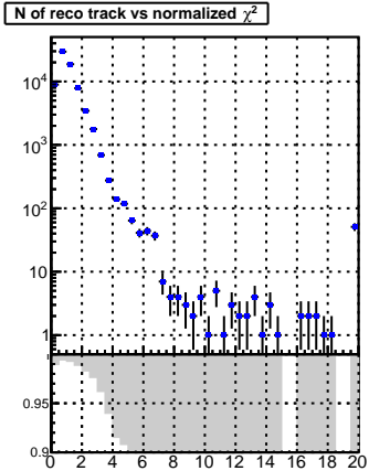
N of reco track vs. \chi^2 tracking_iters01LST_DNN_1000events
