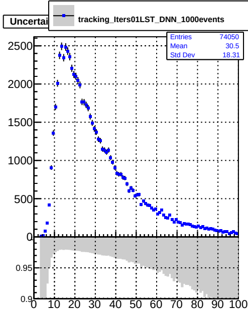
Uncertainty z Coordinate (other Vtx)
