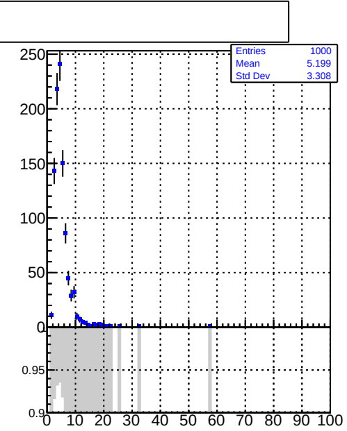
Uncertainty z Coordinate (tagged Vtx)
