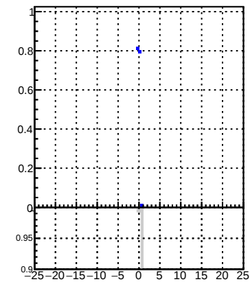
Efficiency vs Dxy(PV) tracking_iters01LST_DNN_1000events
