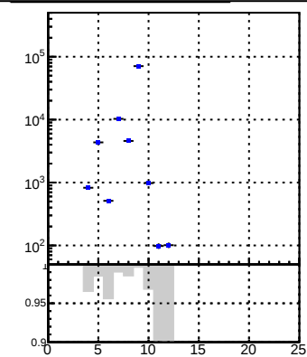
tracking_iters01LST_DNN_1000events
