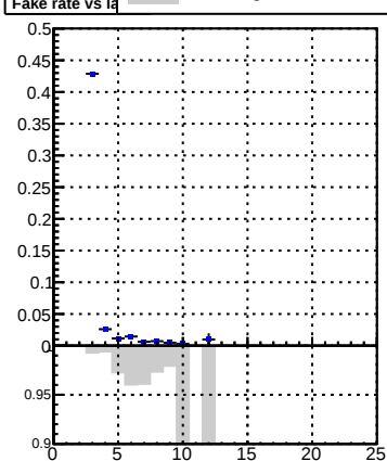
Fake rate vs hit tracking_Iters01LST_DNN_1000events
